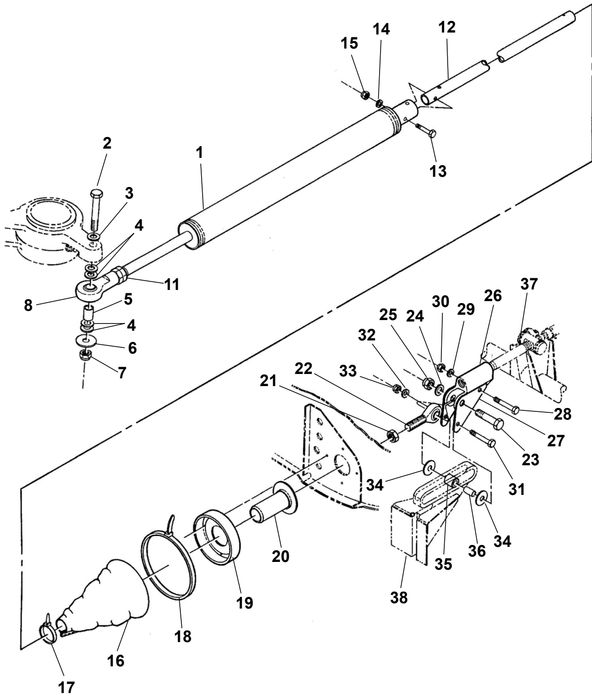
NOSE GEAR STEERING Figure 01. (Sheet 1)
