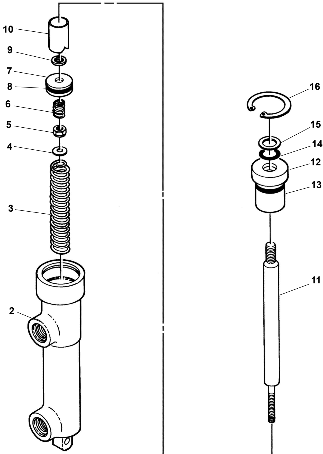
BRAKE MASTER CYLINDER ASSEMBLY Figure 01. (Sheet 1)
