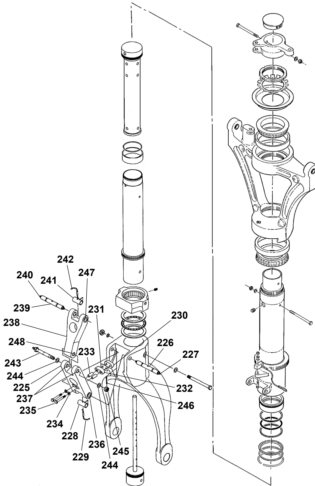
NOSE GEAR SHOCK STRUT ASSEMBLY Figure 02. (Sheet 4)
