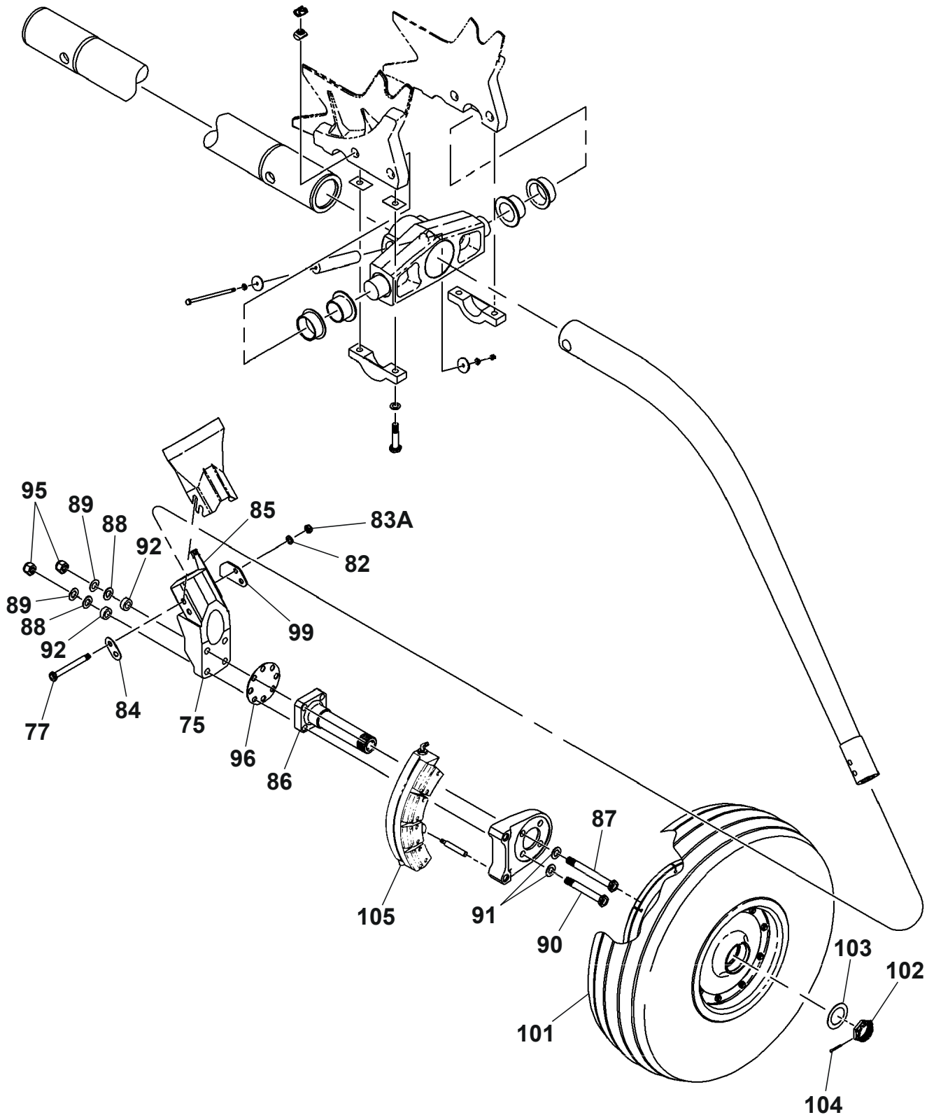
MAIN LANDING GEAR INSTALLATION Figure 01. (Sheet 2)
