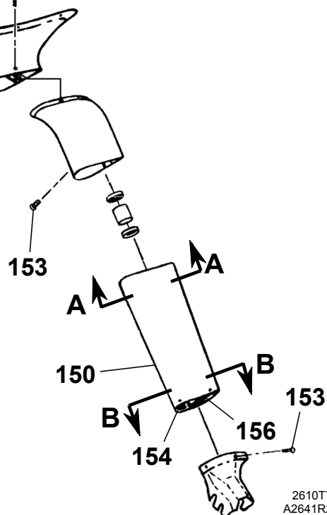
MAIN LANDING GEAR FAIRINGS INSTALLATION Figure 01. (Sheet 3)
