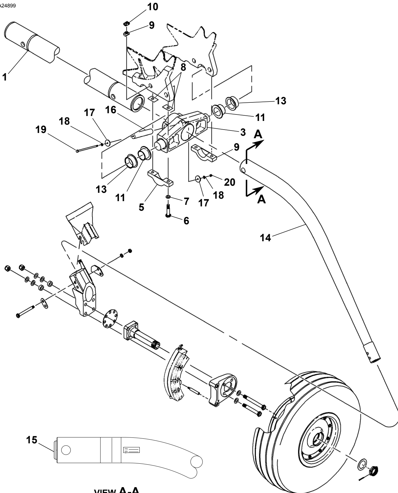
MAIN LANDING GEAR INSTALLATION Figure 01. (Sheet 1)
