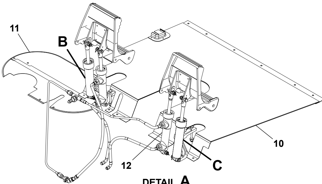
BRAKE RETURN SPRING INSTALLATION Figure 01. (Sheet 1)
