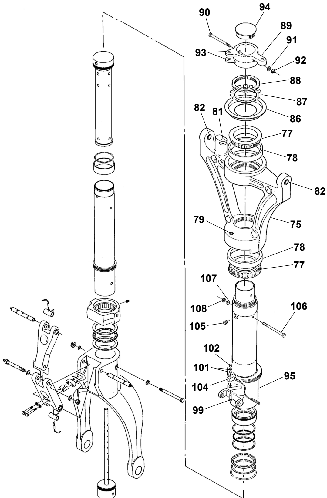
NOSE GEAR SHOCK STRUT ASSEMBLY Figure 02. (Sheet 2)
