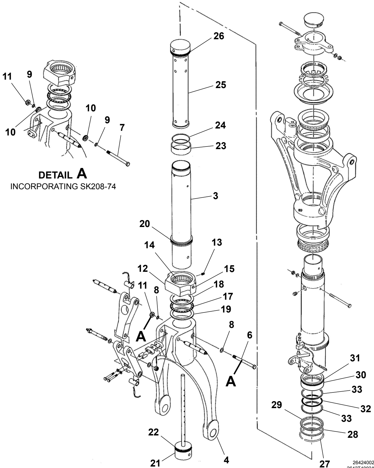
NOSE GEAR SHOCK STRUT ASSEMBLY Figure 02. (Sheet 1)
