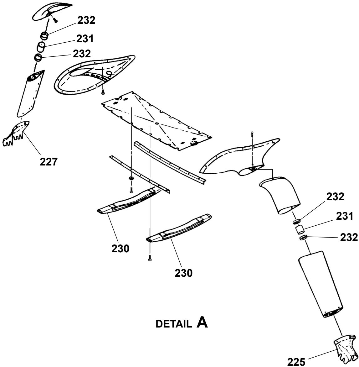
MAIN LANDING GEAR FAIRINGS INSTALLATION Figure 01. (Sheet 4)
